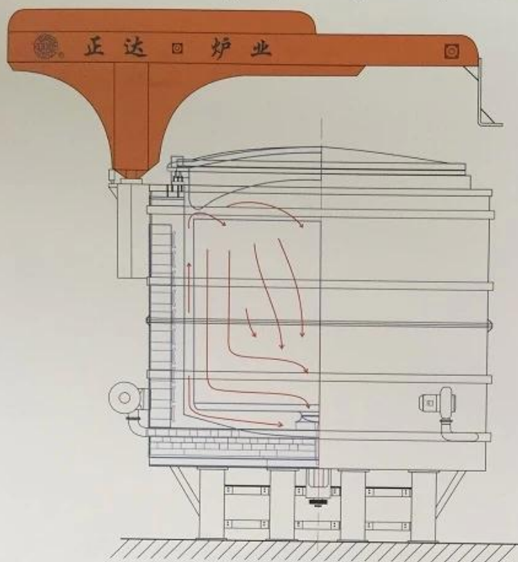
ZD-8355 Type supercon type spheroidizing Annealing furnace schematic diagram
